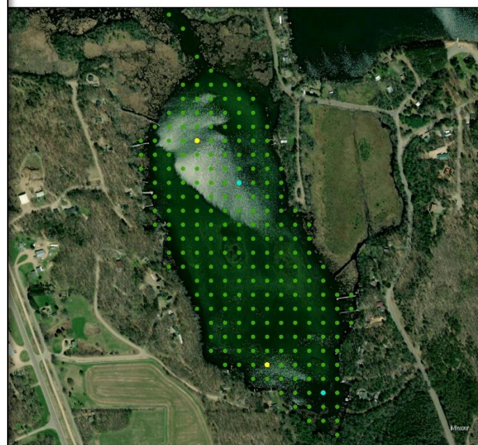
Smoke Lake Aquatic Plant Survey 2020: Total Number of Species
